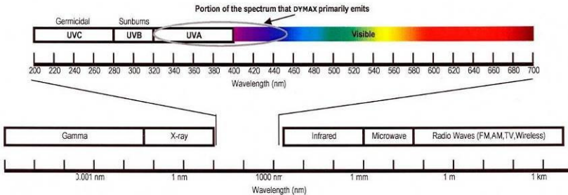
Figure 1. UV Spectrum
