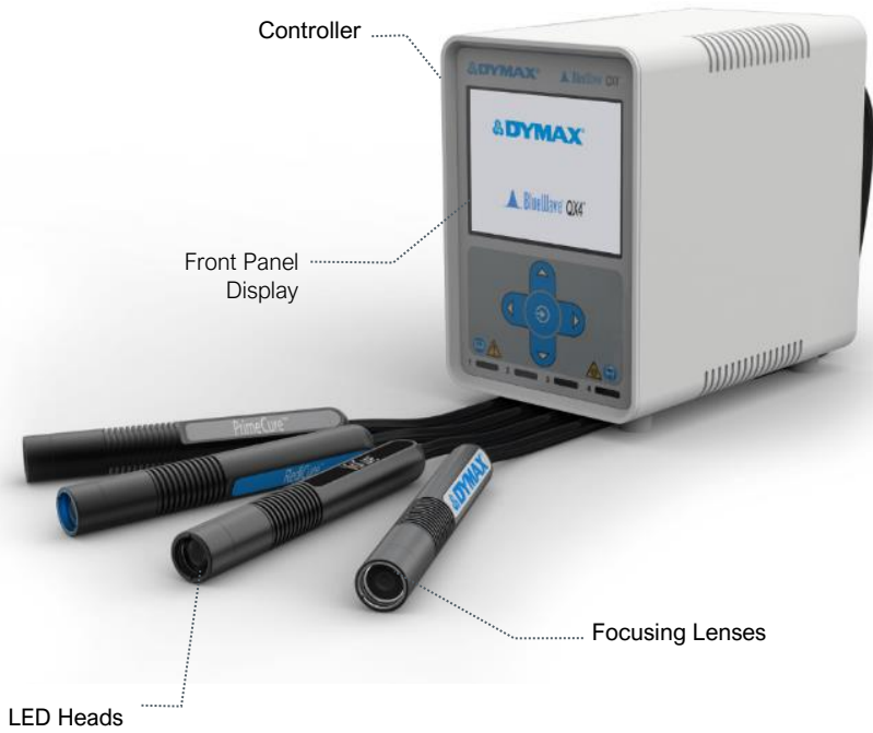
Figure 2. Main Components of a BlueWave QX4
