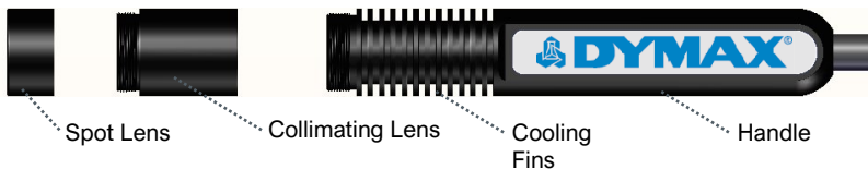
Figure 5. LED Head Components
