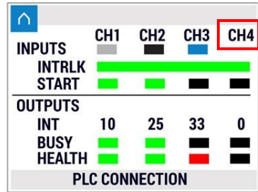
Figure 27. Channel Identifiers
