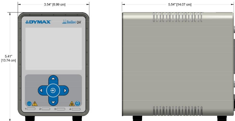
Figure 45. Dimensions - Controller
